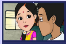
Animated Videos
